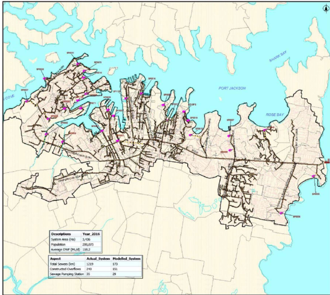
Figure 5-1 Major assets in the Bondi Wastewater DSP area
